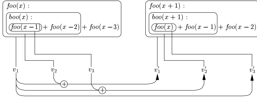
Fig. 6. Transitive dependencies.
